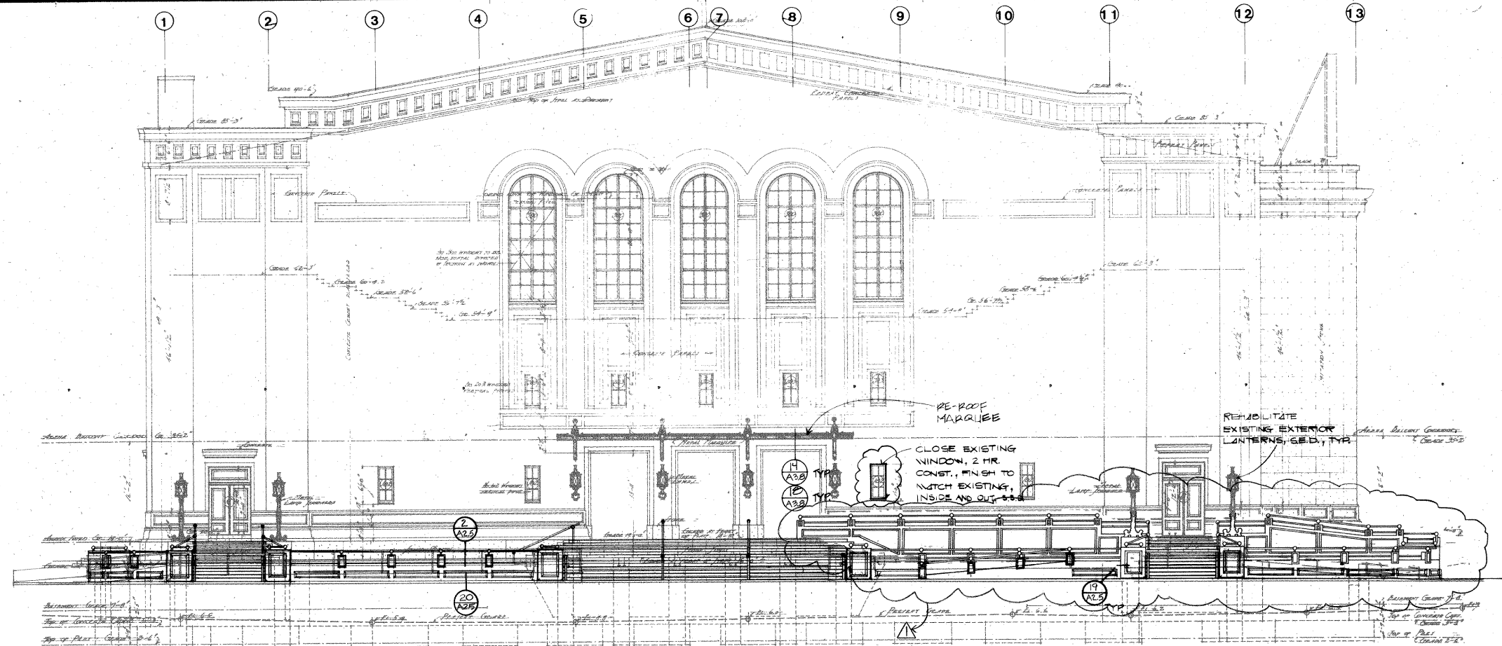
EAST ELEVATION
