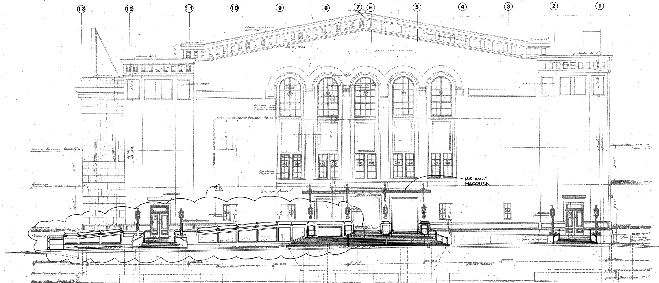
WEST ELEVATION
