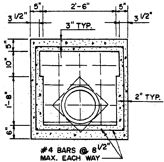
SECTION B
