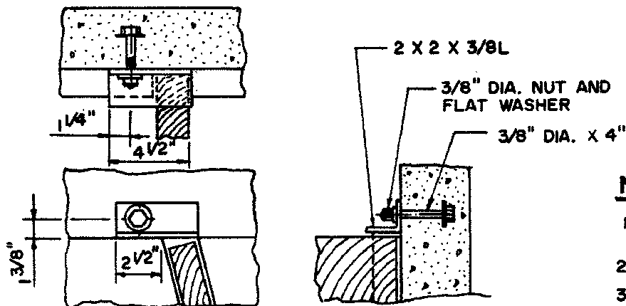
LOCK DETAIL
